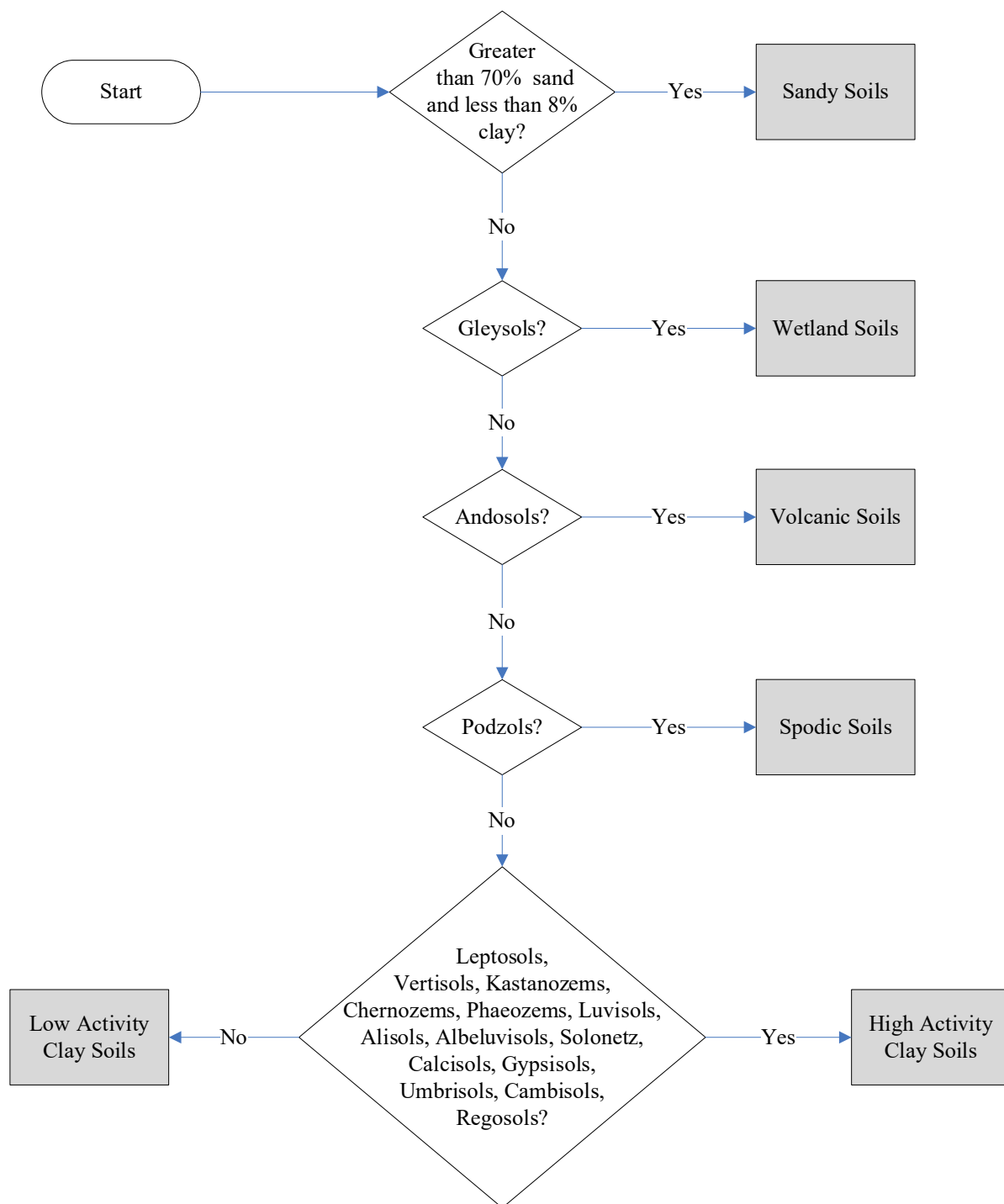
Figure 3A.5.4 Classification scheme for mineral soil types based on World Reference Base for Soil Resources (WRB) classification.
